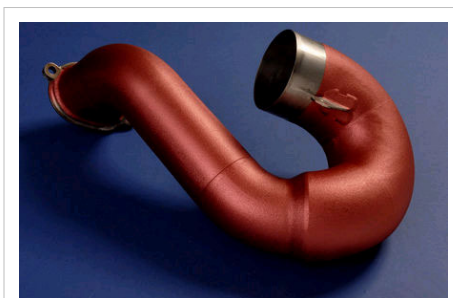
Ceramic is used for its low thermal conductivity on exhaust systems to prevent heat from reaching sensitive components
